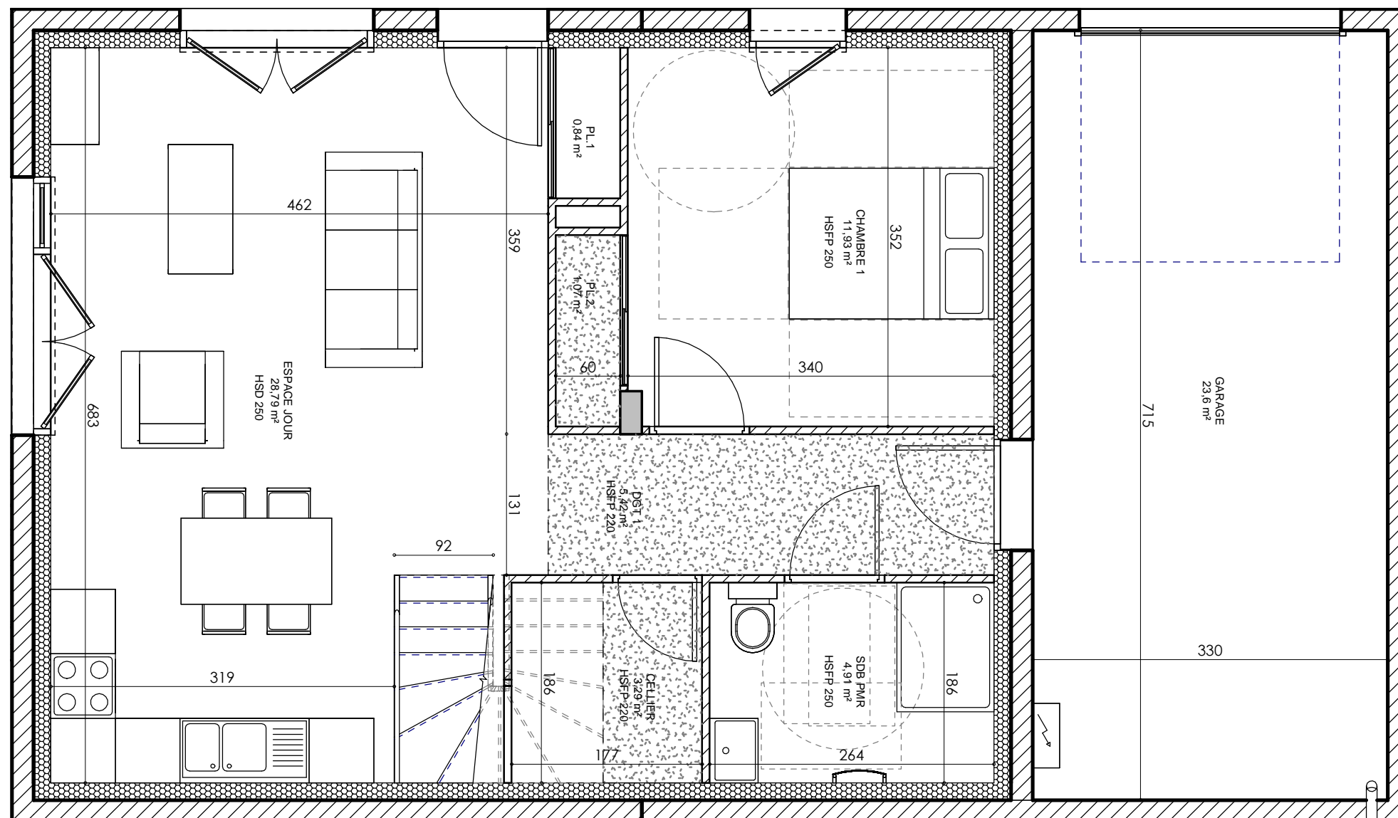
Plan RDC - 1/50
